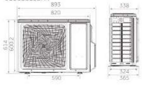
1U50S2SJ2FA
