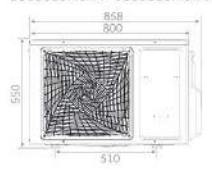
1U25S2SM1FA - 1U35S2SM1FA
